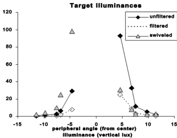
Fig. 4: Vertical illuminances on targets for each headlamp condition.
