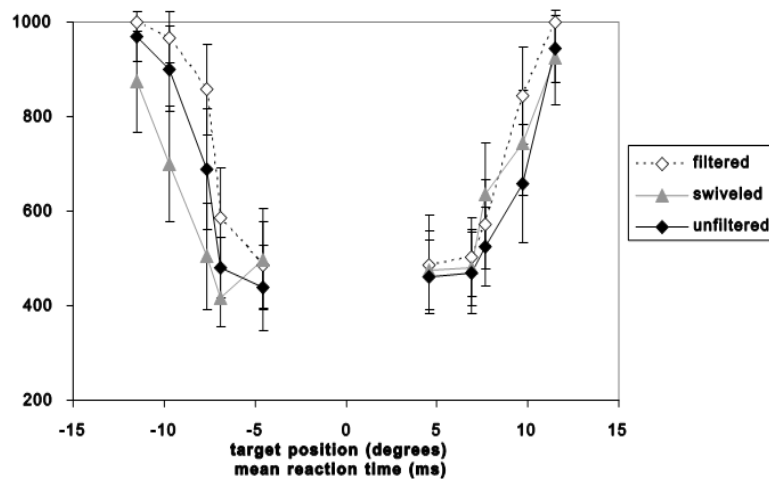
Fig. 6: Missed targets for each target location, target size and headlamp condition.
