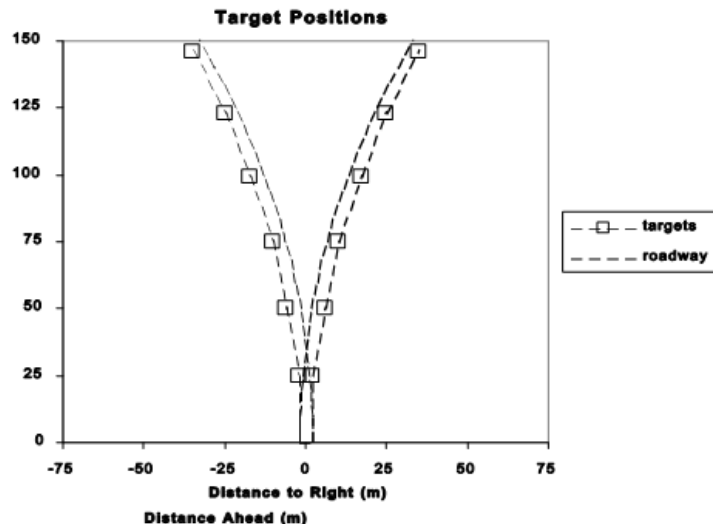
Fig. 1: Layout of roadway curves and location of targets along each side.
